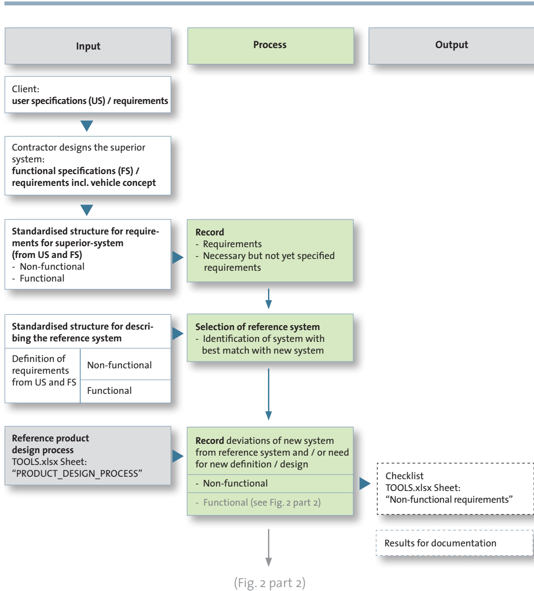
Process steps in the QE process model (Fig. 2 part 1)
